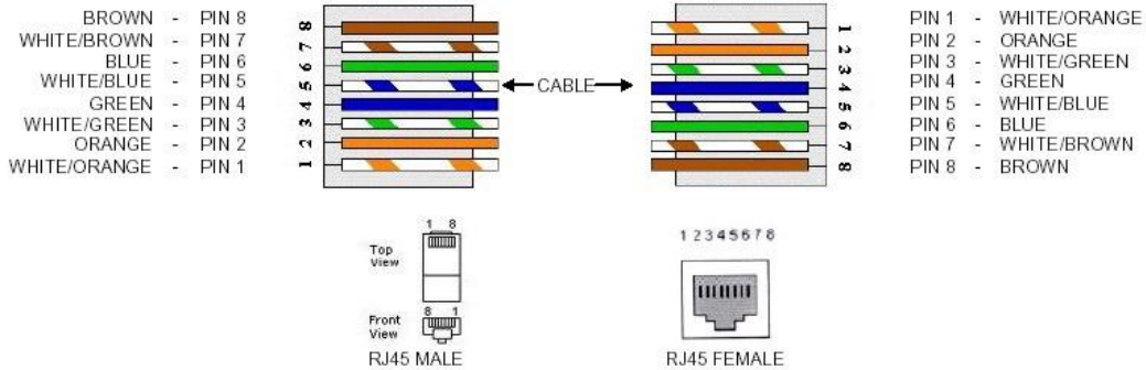
RJ45 (Pin to Pin) Wiring Diagram:
